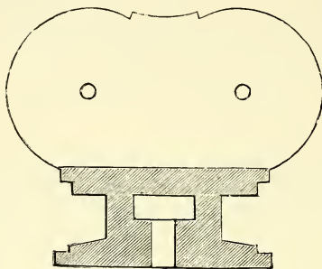
Section of Bar-lock Breech-action.
